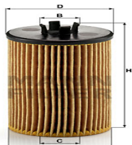
Oil Filter HU 612/2 x EM-10042
